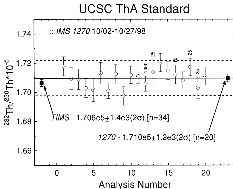
Fig. 3. Replicate ^{232}\text{Th}/^{230}\text{Th} analyses of UCSC ThA standard run with IMS 1270 SIMS in October 1998. All analyses were externally standardized by careful gain matching of FC and EM detectors with ^{232}\text{Th}^+ signal from pure Th metal. Most SIMS analyses were performed on large unconfined loads in carbon. Loads that were confined by polyethylene rings are marked with their load weight in ng adjacent to each symbol. Twenty replicates by SIMS over a 25 day period gave a value of 1.710 \times 10^5 \pm 1.2 \times 10^3 ( 2\sigma ). Also plotted is an independent analysis of UCSC ThA by TIMS ( 1.706 \times 10^5 \pm 1.4 \times 10^3 ( 2\sigma ; n = 34 ); [5]). Other available independent analysis of UCSC ThA include replicate TIMS analyses by Rubin ( 1.709 \times 10^5 \pm 1.6 \times 10^3 ( 2\sigma ; n = 149 ); [17]) and ICP-MS ( 1.708 \times 10^5 \pm 2.6 \times 10^3 ( 2\sigma ; n = 5 ); [5]). All three of these independent analyses agree with the IMS 1270 determination, and with each other, within their stated uncertainties. All tabled standard and rock sample data in this article are referenced to the previously derived SIMS value for UCSC ThA.
