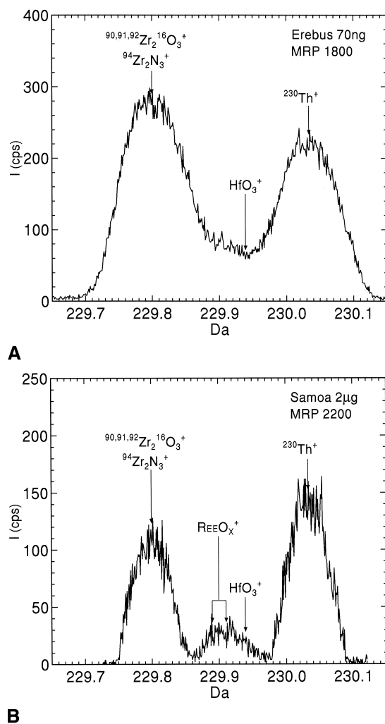
Fig. 2. (A) Mass spectrum of ^{230}\text{Th}^+ and adjacent positive secondary ion peaks in a rock-derived Th load (Erebus 84505 basalt) processed by simple anion exchange. Mass resolving power of 1800 (10% definition) used here is the minimum normal instrument setting. Most analyses are now routinely performed with MRP of 2000–2200. (B) Mass spectrum of ^{230}\text{Th}^+ and adjacent positive secondary ion peaks in a rock-derived Th load (Samoa basalt) processed by TRUSpec/Anion Exchange. MRP was 2200.
