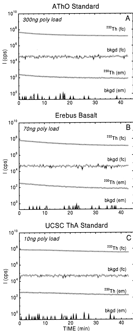
Fig. 1. Relative performance of polyethylene confined sample loads of; (A) ATHO rock standard (300 ng total Th), (B) Erebus 84505 basalt sample (70 ng total Th), and (C) UCSC ThA synthetic standard (10 ng total Th). Signal intensity ( I ) is expressed in counts per second (cps) for each individual counting cycle. Both electron multiplier (EM) and Faraday Cup detectors (FC) were used. This set of data demonstrates the relative independence of I on total Th content of sample, implying instead that a rather consistent aliquot of Th is consumed in each analysis. This is attributed to the generation, for each sample analysis, of a generally consistent sputter crater size in a relatively uniformly porous carbon medium hosting the Th.
